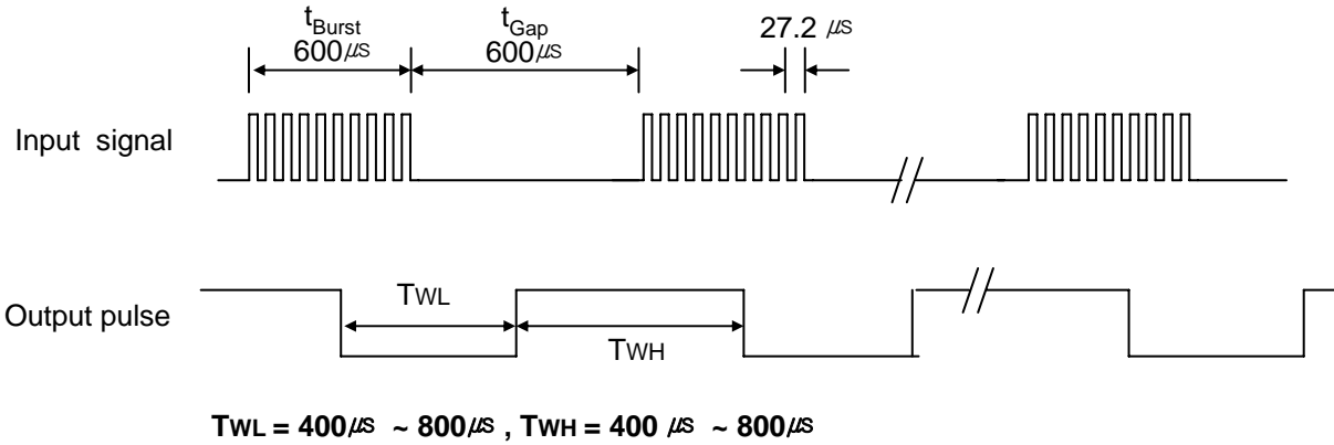
[ Fig.1 ] Output Waveform ( at freq.=36.7KHz )
